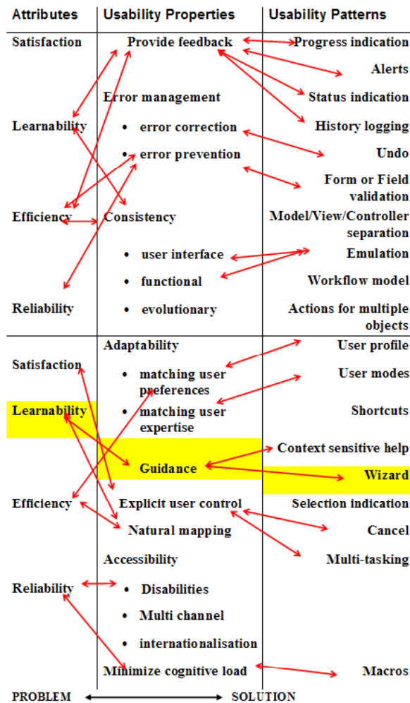
Figure 1: Usability Framework
